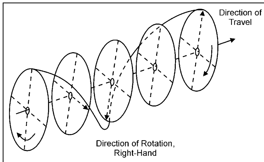
Figure 8-6. Circular polarization
