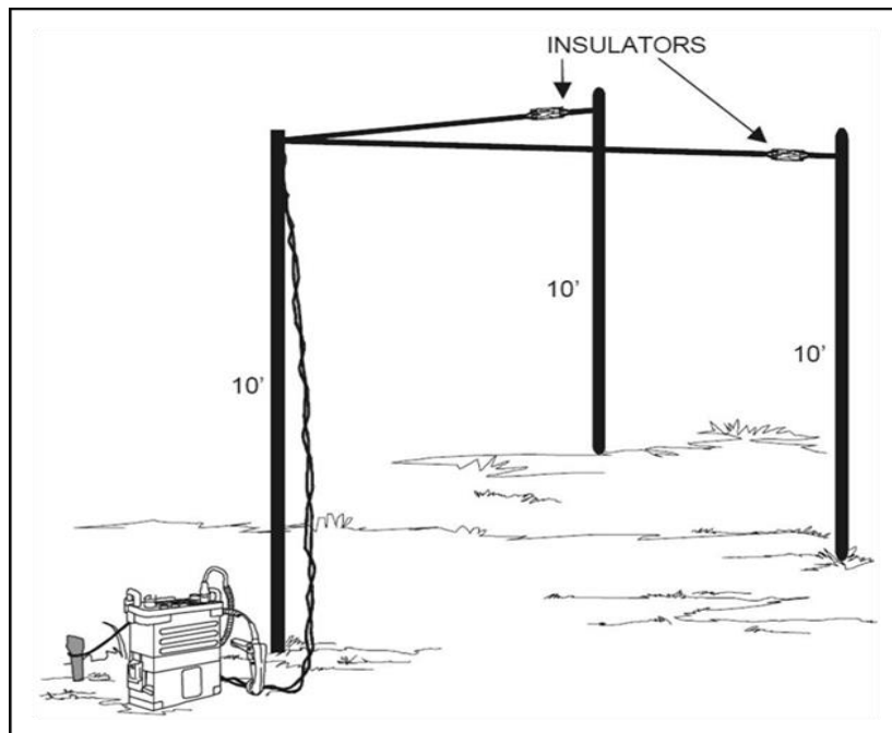
Figure 8-13. V antenna
