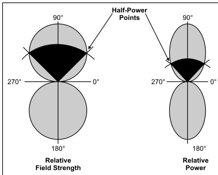
Figure 8-10. Beamwidth
