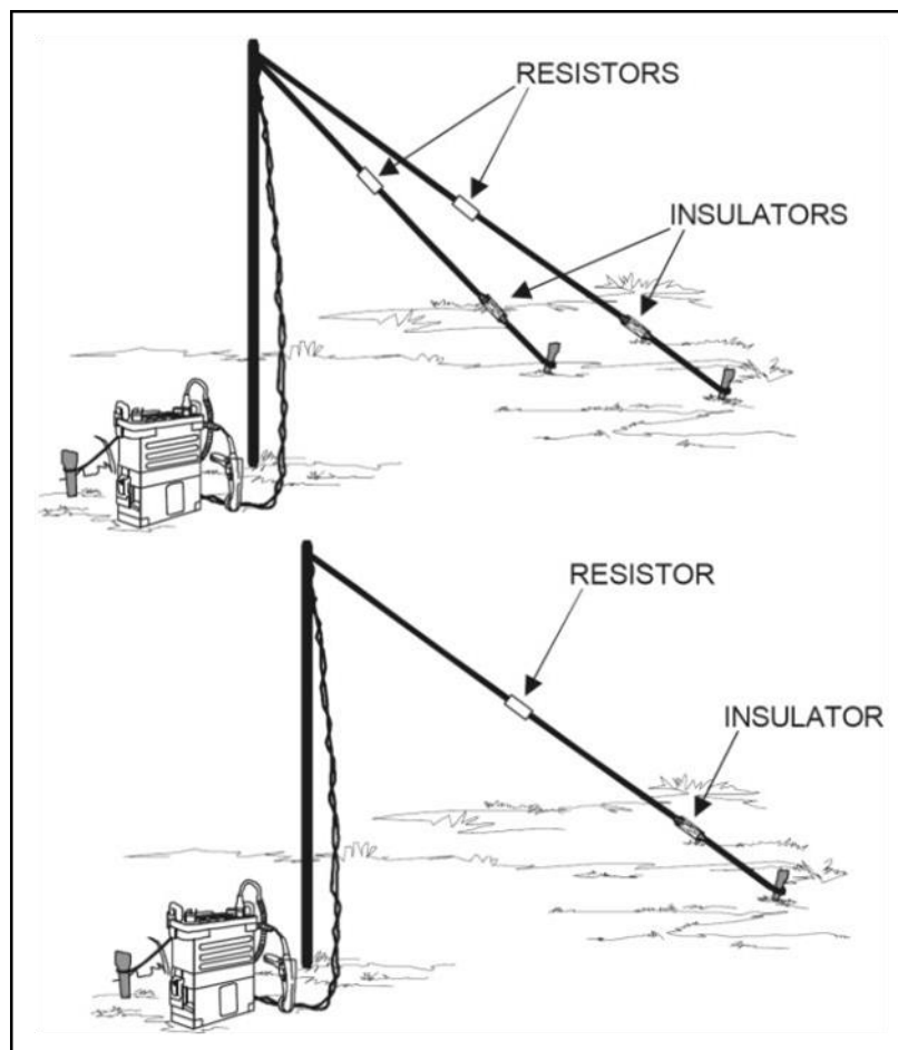
Figure 8-16. Sloping-V antenna
