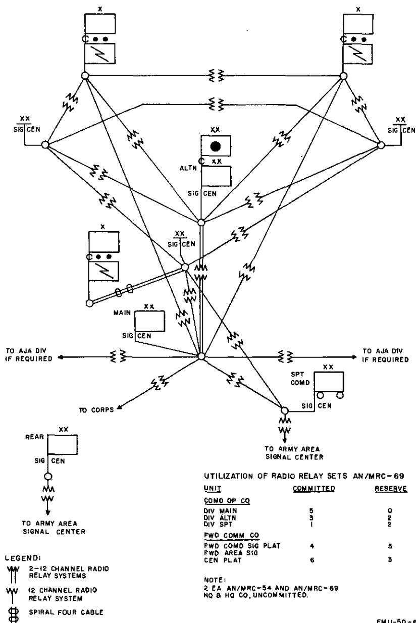
Figure 5. Type multichannel communication network for the offense.
