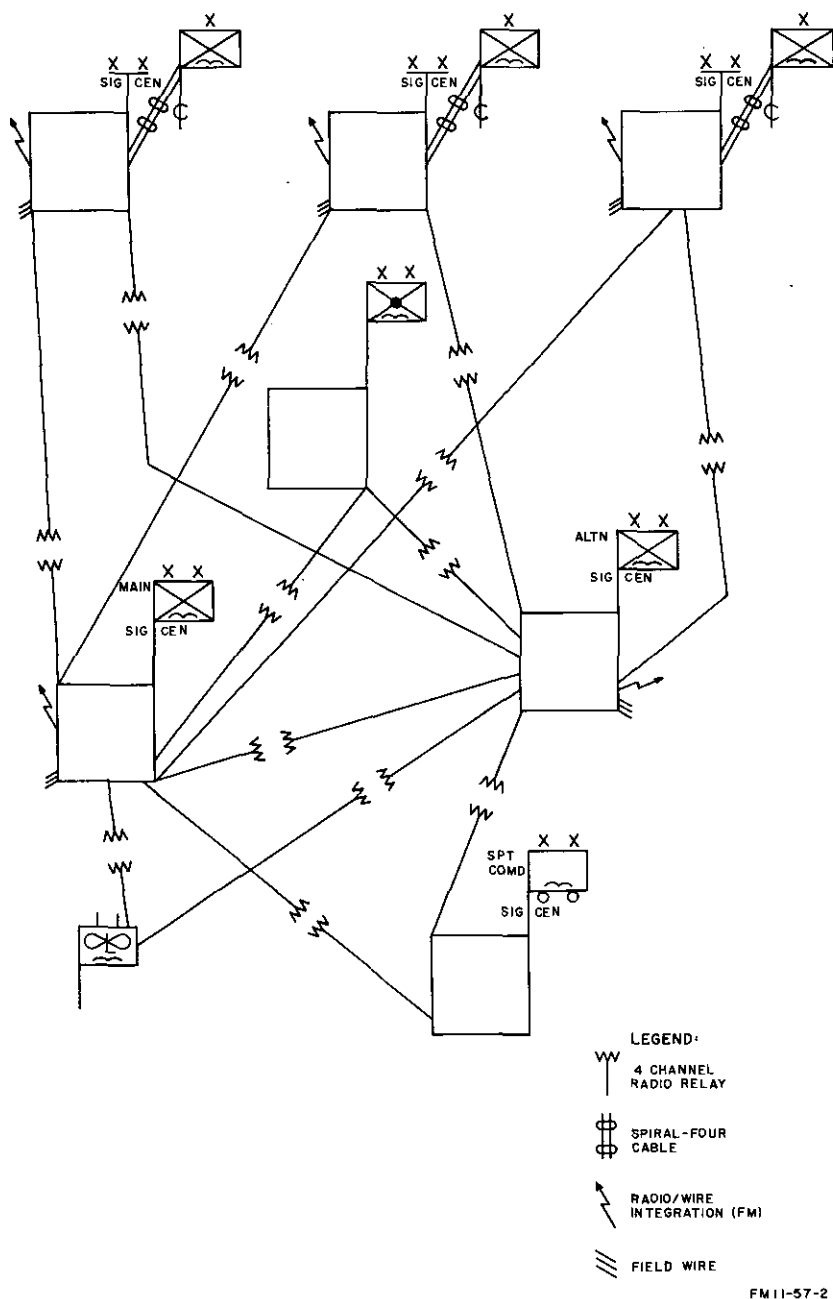
Figure 8. Type airborne division multichannel communication network.
