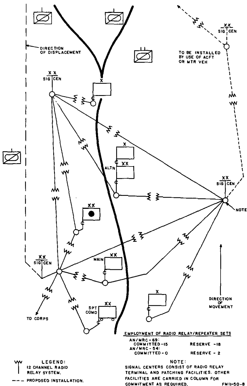
Figure 7. Type multichannel communication network for the advance to contact.
