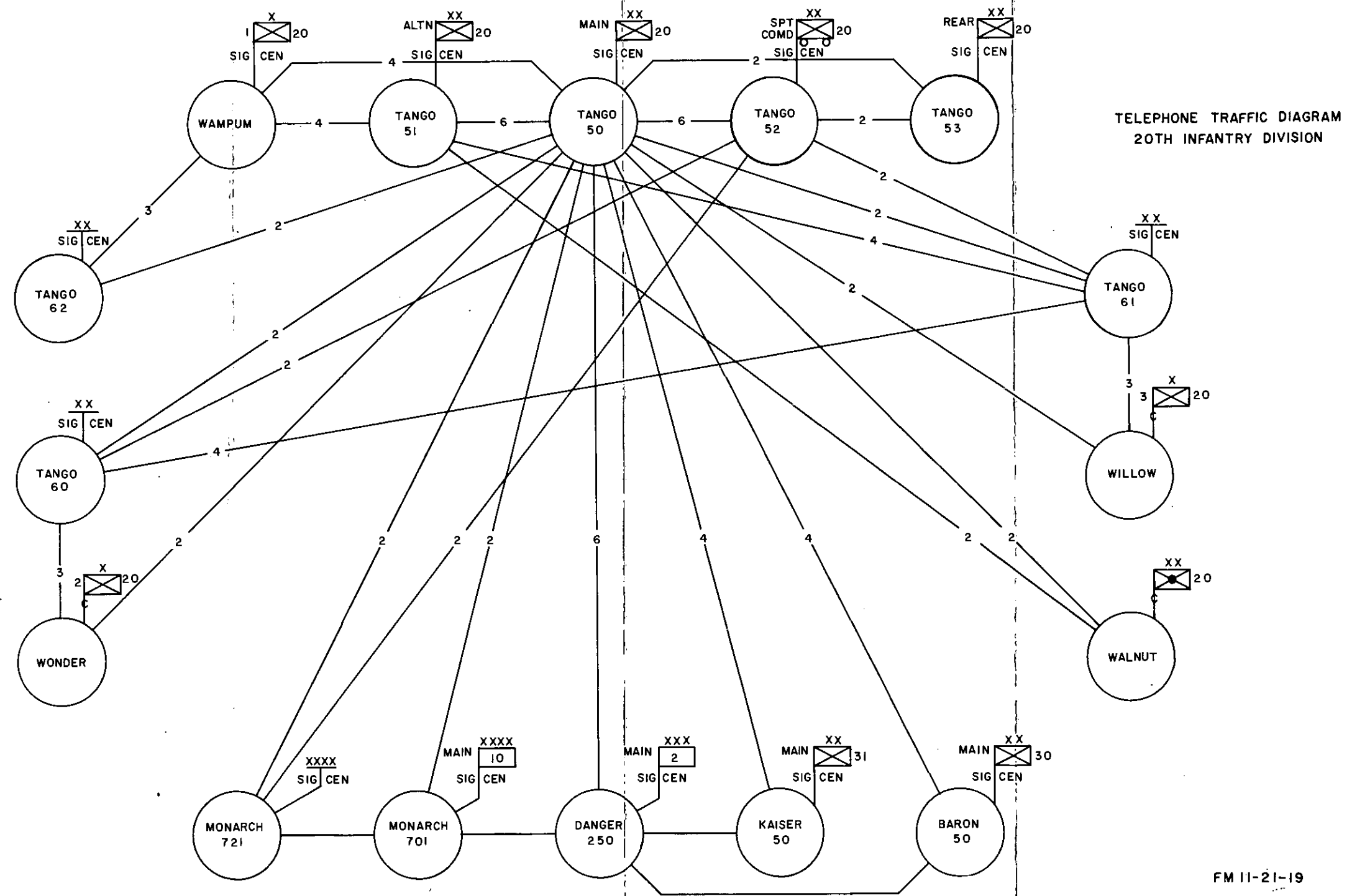
Figure 13. Type infantry division telephone traffic diagram.
