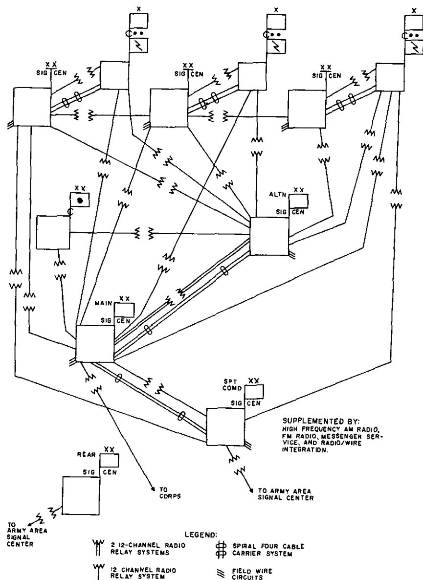
Figure 4. Type division area communication system.
