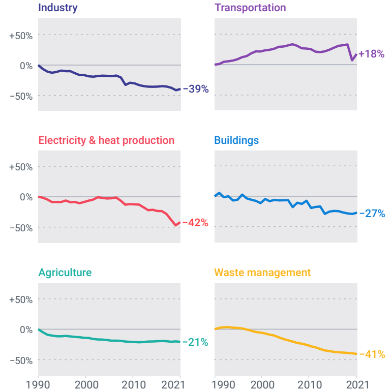
EMISSIONS TRENDS PER SECTOR as compared to 1990
