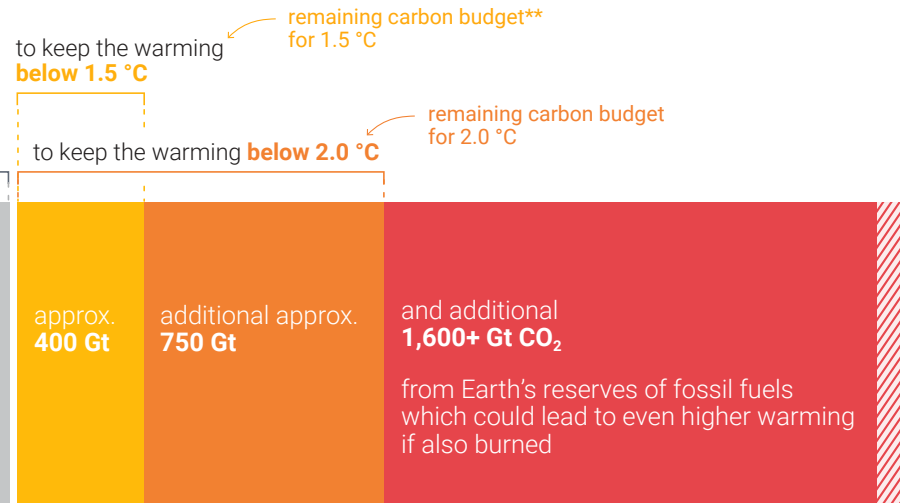
Global CO 2 emissions from further combustion of fossil fuels
