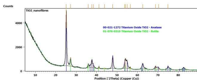
Figure 1: Depicts the XRD spectra of \text{TiO}_2 nanofibers
