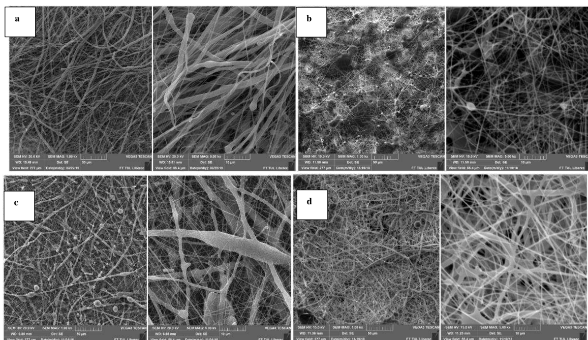
Figure 1: SEM image of pure PCL electrospun layer (a); pure PVA electrospun layer (b); PCL/PVA hybrid layer from dual jet spinning (c); PCL/PVA hybrid layer from needleless electrospinning (d).
