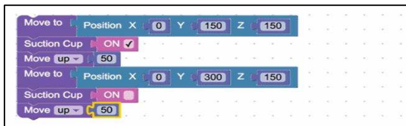
Figure 2. User interface (Blockly)
