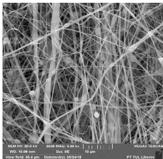
Figure 1: A sample of PVA nanofibers prepared from 12 wt.% precursor solution.
