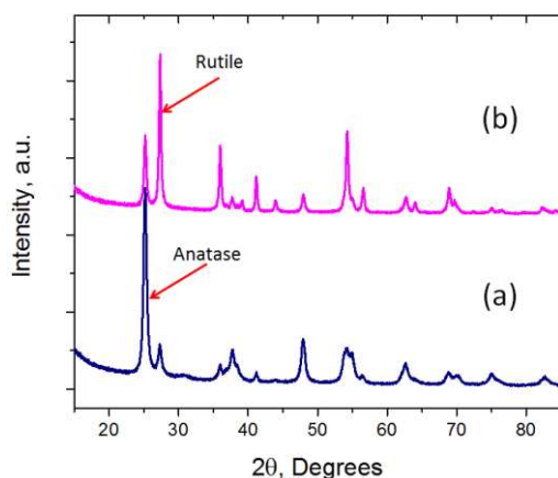
Figure 1. XRD patterns of (a) anatase-rich and (b) rutile-rich titania nanofibers prepared by AC-electrospinning and heat treated at 500°C.
