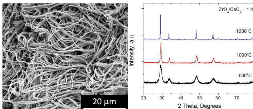
Figure 1. SEM image (left) and XRD patterns at different temperatures (right) of \text{ZrO}_2/\text{CeO}_2 composite nanofibers with 1:4 molar ratio.
