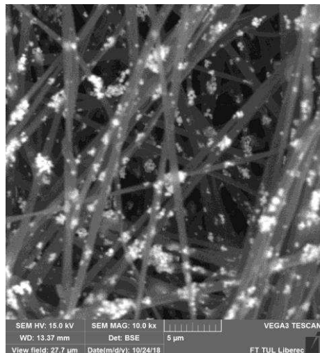
Figure 1: SEM image of electrospun PVB/ Bi 2 O 3 in ratio 1:1 (material contrast).
