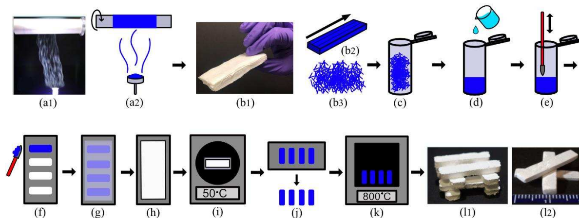
Figure 1: Process of making (3-D) glass-ceramic fibrous structures.
