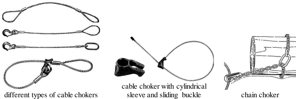
Fig. 63. Chokers
