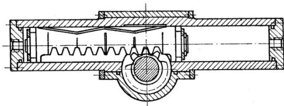
Fig. 40. Hydraulic motor with toothed rack and pinion (the principle is used e.g. for slewing mechanisms of hydraulic cranes) (Bauer, Ryšavý, 1985)
