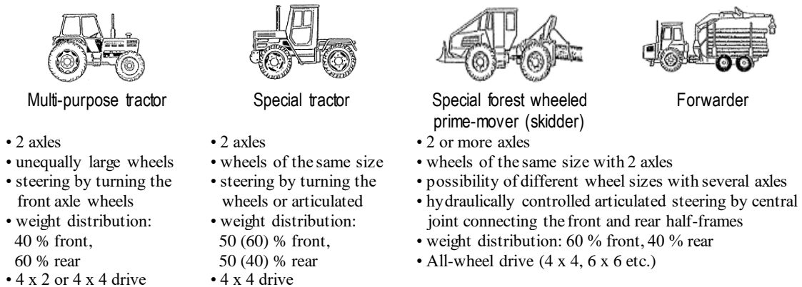
Fig. 1. Distinction of wheeled tractors and prime-movers
